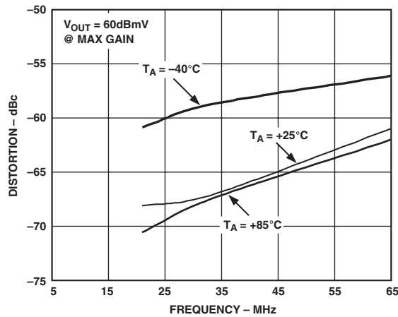
TPC 2. Second-Order Harmonic Distortion vs. Frequency vs. Temperature
