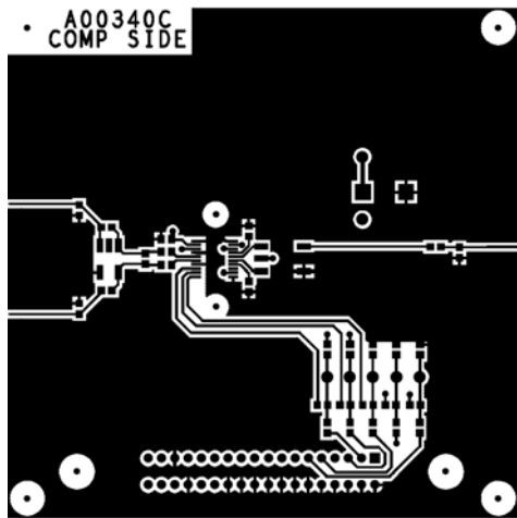
Figure 12. Primary Side
