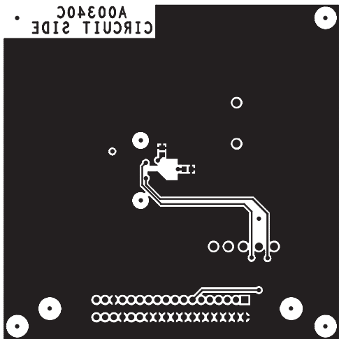
Figure 16. Secondary Side
