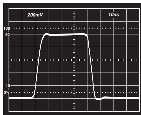
Figure 9. Pulse Response for the Circuit of Figure 8
