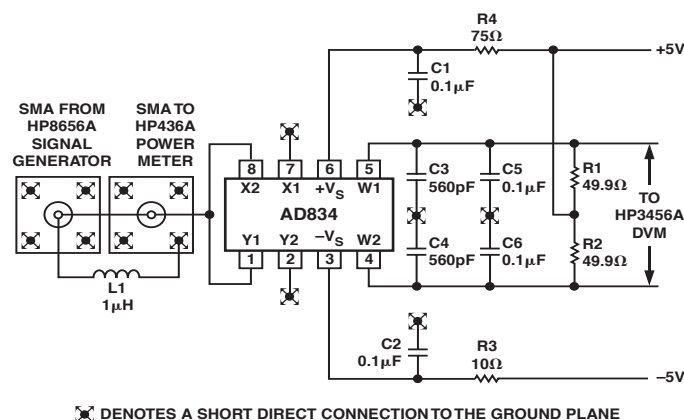
Figure 2. Bandwidth Test Circuit
