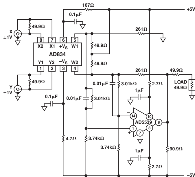
Figure 8. Sideband DC-Coupled Multiplier
