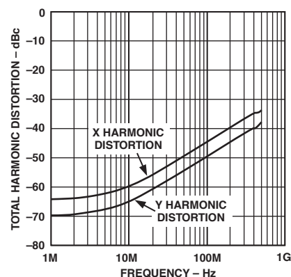
TPC 3. Total Harmonic Distortion vs. Frequency
