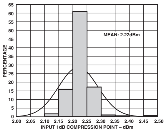
TPC 27. Input 1 dB Compression Point Histogram f_{IN} = 2400 MHz, f_{OUT} = 425 MHz
