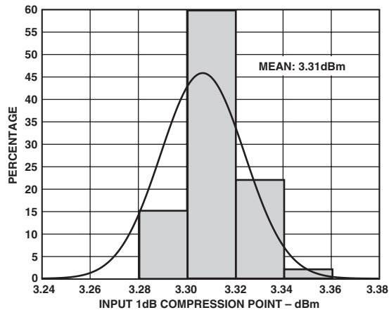
TPC 3. Input 1 dB Compression Point Histogram f_{IN} = 400 MHz, f_{OUT} = 70 MHz
