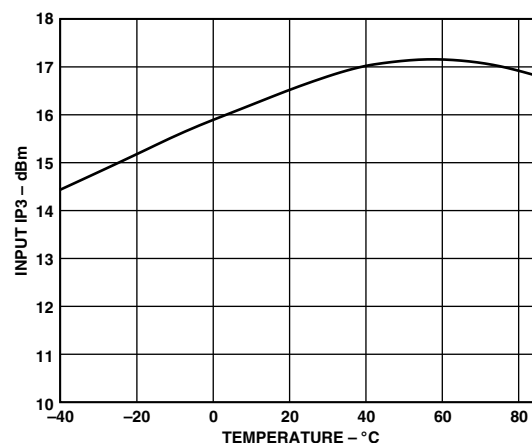
TPC 29. Input IP3 Performance Over Temperature f_{IN} = 2400 MHz, f_{OUT} = 425 MHz
