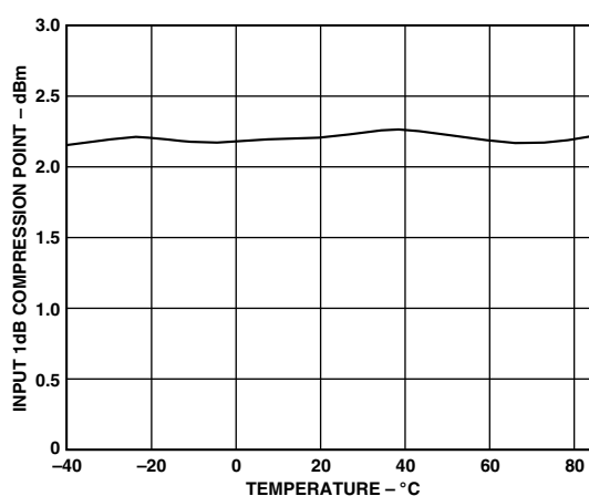
TPC 30. Input 1 dB Compression Point Performance Over Temperature f_{IN} = 2400 MHz, f_{OUT} = 425 MHz
