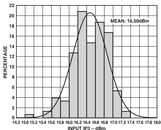
TPC 26. Input IP3 Histogram f_{IN} = 2400 MHz, f_{OUT} = 425 MHz
