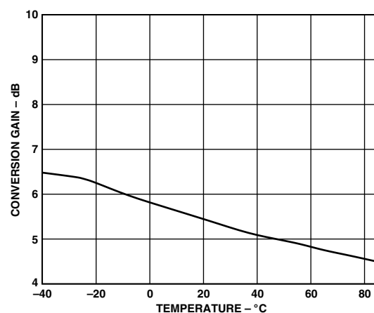
TPC 28. Gain Performance Over Temperature f_{IN} = 2400 MHz, f_{OUT} = 425 MHz
