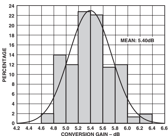
TPC 25. Gain Histogram f_{IN} = 2400 MHz, f_{OUT} = 425 MHz
