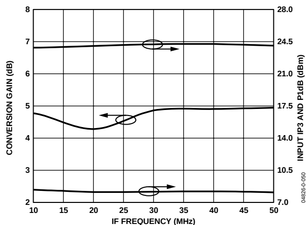
Figure 47. Conversion Gain, Input IP3, and P1dB vs. IF Frequency, F_{RF} = 890 MHz
