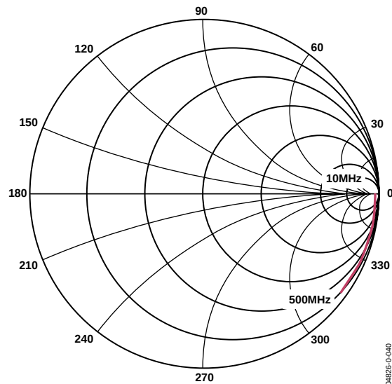
Figure 37. IF Port Reflection Coefficient from 10 MHz to 500 MHz
