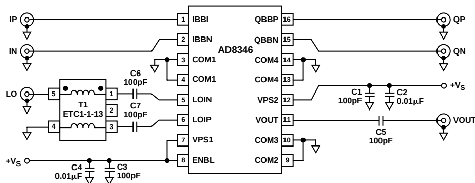
Figure 21. Basic Connections
