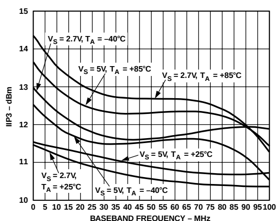
TPC 12. IIP3 vs. F_{BB} , V_{GIN} = 1.2 V , F_{LO} = 1900 \text{ MHz}
