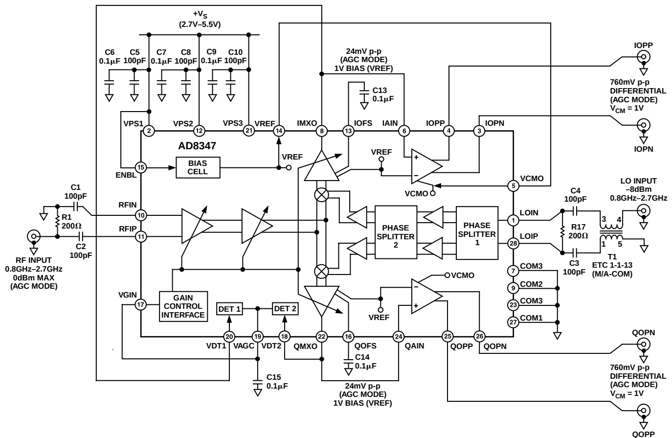
Figure 4. Basic Connections
