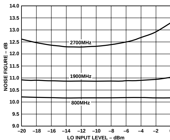
TPC 17b. Noise Figure vs. LO Input Level, Temperature = 25°C, V_{GIN} = 0.2\text{ V} , V_S = 5\text{ V}
