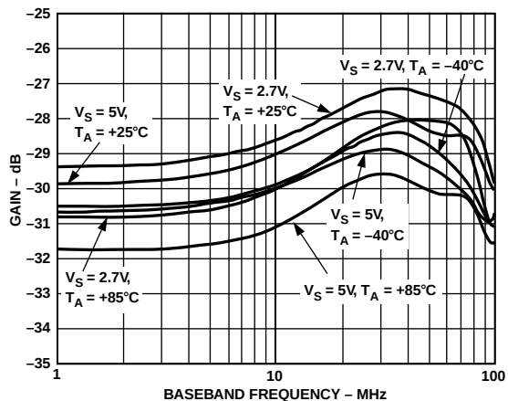
TPC 8. Gain vs. F_{BB} , V_{GIN} = 1.2 V , F_{LO} = 1900 \text{ MHz}
