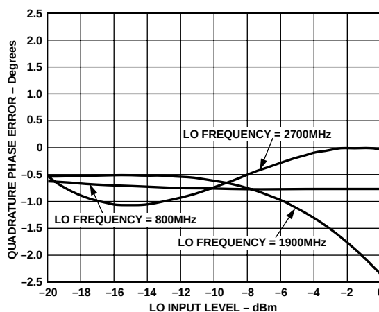
TPC 17a. Quadrature Error vs. LO Power Level, Temperature = 25°C, V_{GIN} = 0.2\text{ V} , V_S = 5\text{ V}
