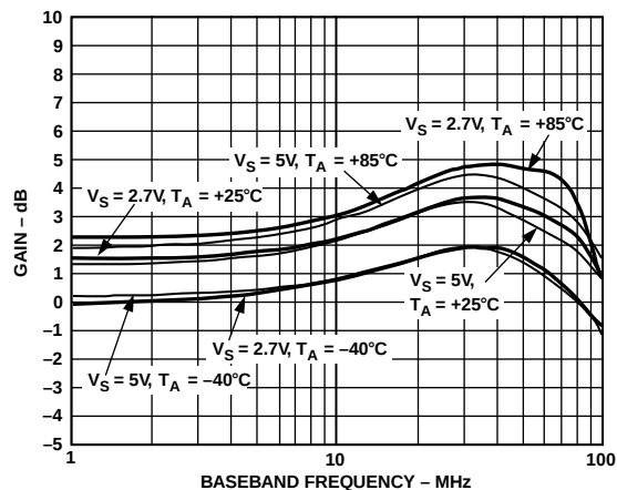
TPC 7. Gain vs. F_{BB} , V_{GIN} = 0.7 V , F_{LO} = 1900 \text{ MHz}
