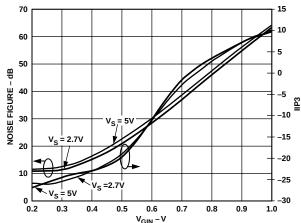
TPC 16. Noise Figure and IIP3 vs. V_{GIN} , Temperature = 25°C, F_{LO} = 1900\text{ MHz} , F_{BB} = 1\text{ MHz}
