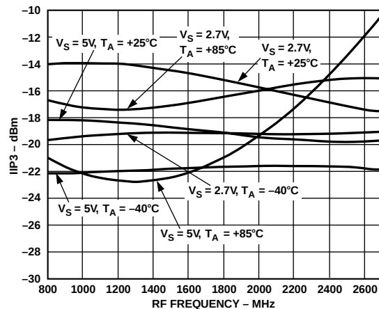
TPC 11. IIP3 vs. F_{LO} , V_{GIN} = 0.2 V , F_{BB} = 1 \text{ MHz} ,
