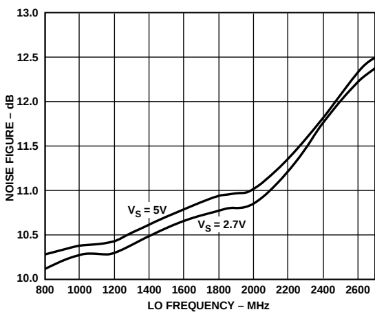
TPC 15. Noise Figure vs. LO Frequency ( F_{LO} ), Temperature = 25°C, V_{GIN} = 0.2\text{ V} , F_{BB} = 1\text{ MHz}
