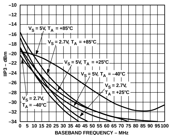
TPC 13. IIP3 vs. F_{BB} , V_{GIN} = 0.2\text{ V} , F_{LO} = 1900\text{ MHz}
