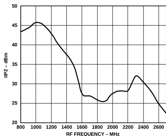
TPC 14. IIP2 vs. F_{LO} , V_{GIN} = 1.2\text{ V} , Baseband Tone1 = 5 MHz, -10 dBm, Baseband Tone2 = 6 MHz, -10 dBm, Temperature = 25°C, V_S = 5\text{ V}
