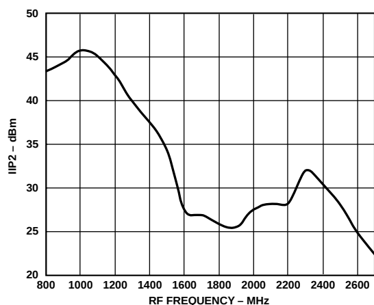
TPC 14. IIP2 vs. F_{LO} , V_{GIN} = 1.2\text{ V} , Baseband Tone1 = 5\text{ MHz} , -10\text{ dBm} , Baseband Tone2 = 6\text{ MHz} , -10\text{ dBm} , Temperature = 25^\circ\text{C} , V_S = 5\text{ V}
