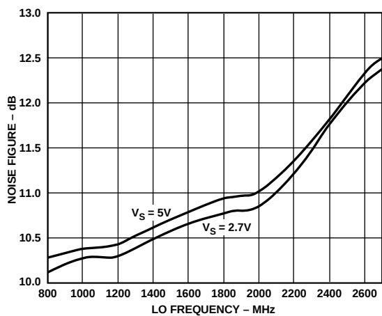
TPC 15. Noise Figure vs. LO Frequency ( F_{LO} ), Temperature = 25^\circ\text{C} , V_{GIN} = 0.2\text{ V} , F_{BB} = 1\text{ MHz}
