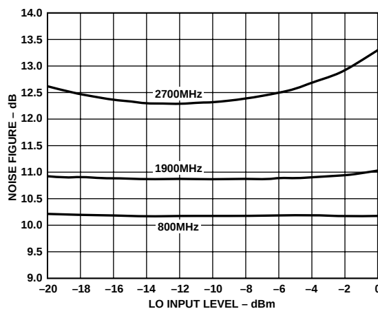
TPC 17b. Noise Figure vs. LO Input Level, Temperature = 25^\circ\text{C} , V_{GIN} = 0.2\text{ V} , V_S = 5\text{ V}
