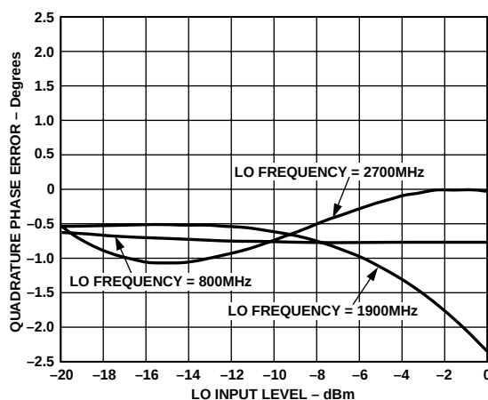
TPC 17a. Quadrature Error vs. LO Power Level, Temperature = 25^\circ\text{C} , V_{GIN} = 0.2\text{ V} , V_S = 5\text{ V}
