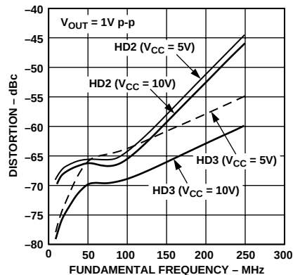
Figure 11. AD8350-20 Harmonic Distortion vs. Frequency
