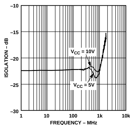
Figure 9. AD8350-20 Isolation ( S_{12} ) vs. Frequency
