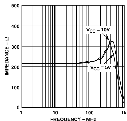
Figure 6. AD8350-15 Output Impedance vs. Frequency
