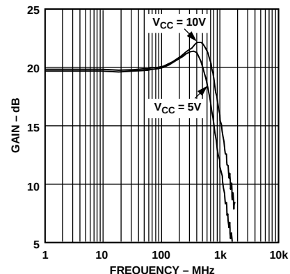
Figure 3. AD8350-20 Gain ( S_{21} ) vs. Frequency
