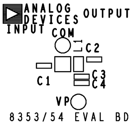
Figure 4. Silkscreen Top
