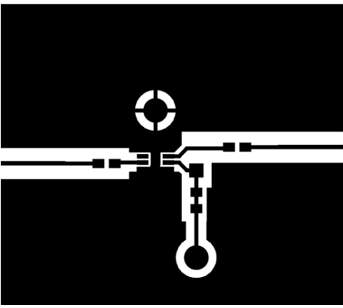
Figure 5. Component Side
