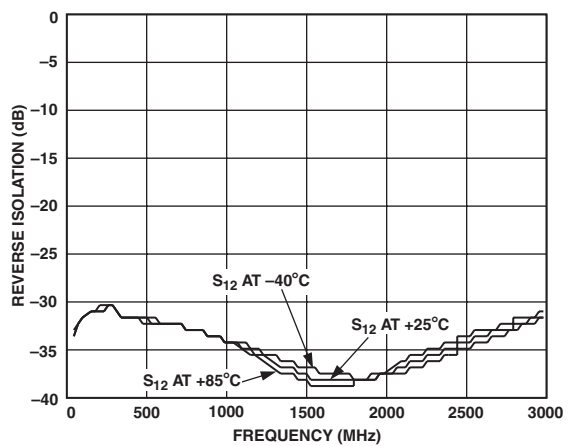
TPC 6. Reverse Isolation vs. Frequency, V_S = 3 V, T_A = -40^\circ\text{C} , +25^\circ\text{C} , and +85^\circ\text{C}
