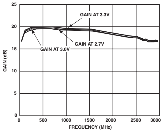
TPC 2. Gain vs. Frequency, V_S = 2.7 V, 3.0 V, and 3.3 V, T_A = 25^\circ\text{C}
