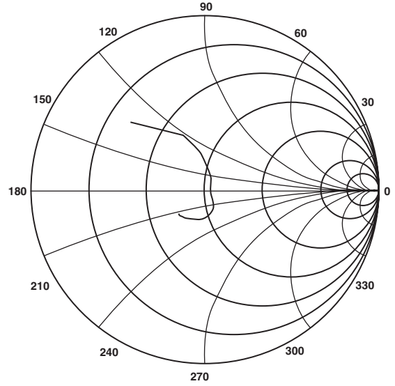
TPC 4. S_{22} vs. Frequency, V_S = 3 V, T_A = 25^\circ\text{C} , 100\text{ MHz} \leq f \leq 3.0\text{ GHz}
