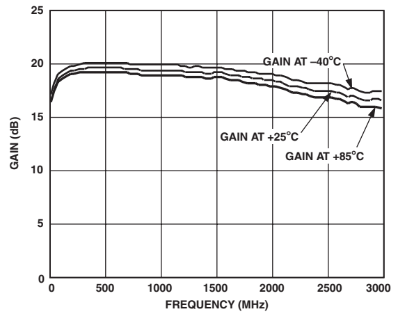
TPC 5. Gain vs. Frequency, V_S = 3 V, T_A = -40^\circ\text{C} , +25^\circ\text{C} , and +85^\circ\text{C}
