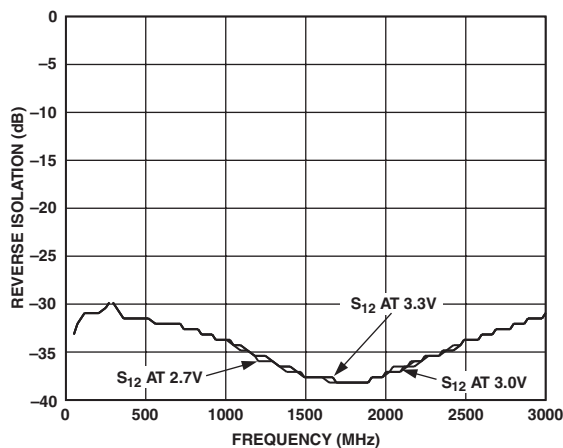
TPC 3. Reverse Isolation vs. Frequency, V_S = 2.7 V, 3 V, and 3.3 V, T_A = 25^\circ\text{C}
