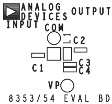
Figure 4. Silkscreen Top
