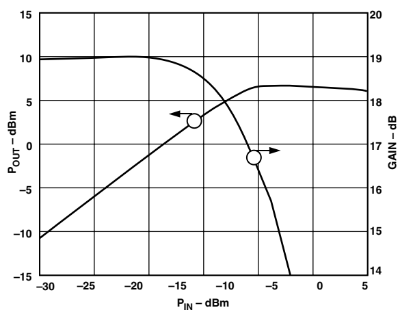
TPC 34. Output Power and Gain vs. Input Power, V_S = 5\text{ V} , T_A = 25^\circ\text{C} , f = 900\text{ MHz}
