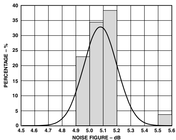
TPC 31. Distribution of Noise Figure, V_S = 5\text{ V} , T_A = 25^\circ\text{C} , f = 2.2\text{ GHz}
