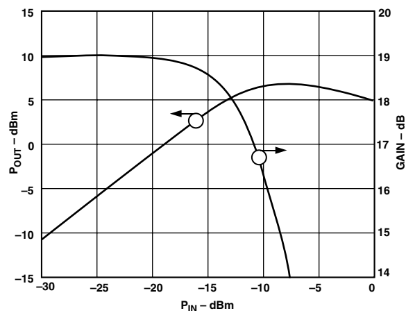
TPC 33. Output Power and Gain vs. Input Power, V_S = 3\text{ V} , T_A = 25^\circ\text{C} , f = 900\text{ MHz}
