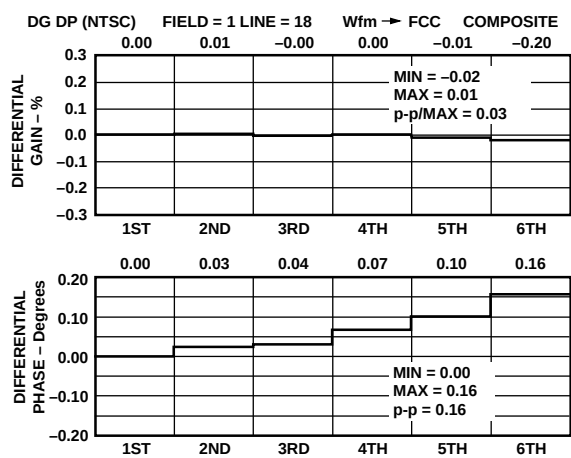
Figure 2. Typical Composite Output Differential Gain & Phase, NTSC for Y Channel; f = 3.58 MHz, R_L = 150 \Omega
