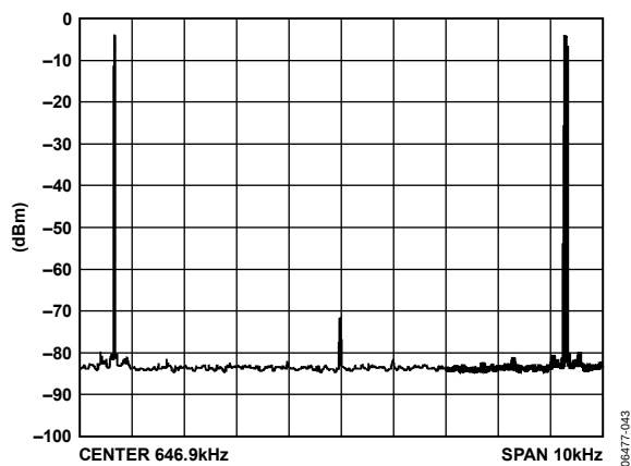
Figure 19. MTPR at 647 kHz
