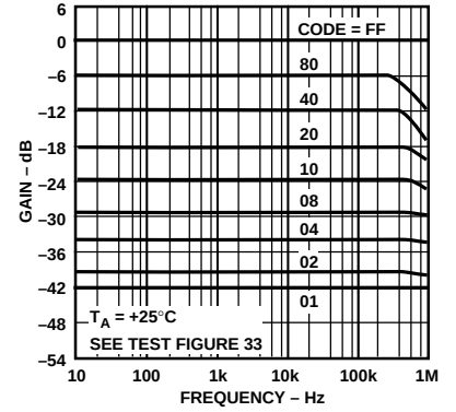
Figure 13. Gain vs. Frequency for R = 10\text{ k}\Omega
