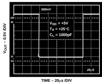
Figure 20. DAC Output Swing with Capacitive Load
