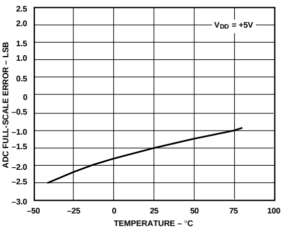
Figure 13. ADC Full-Scale Error vs. Temperature
