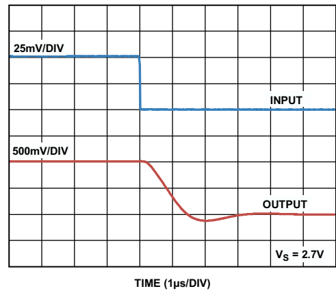
Figure 12. Fall Time ( V_S = 2.7\text{ V} )
