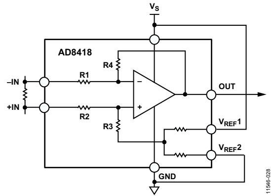
Figure 30. Split Supply
