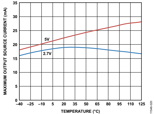
Figure 20. Maximum Output Source Current vs. Temperature
