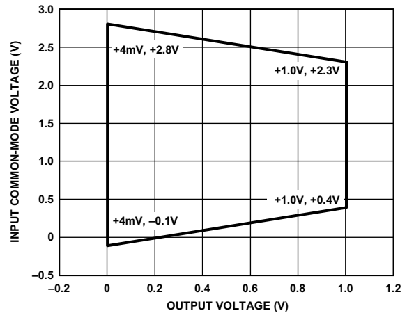
Figure 14. Input Common-Mode Voltage vs. Output Voltage, G = 1 , V_S = 5V
