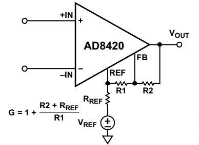
Figure 63. Calculating Gain with Reference Resistance
