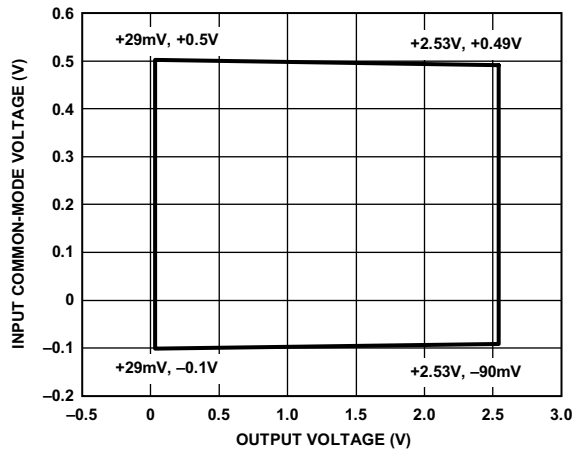
Figure 20. Input Common-Mode Voltage vs. Output Voltage, G = 100 , V_S = 2.7\text{ V}
