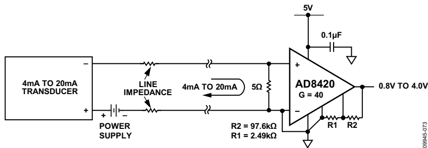
Figure 71. 4 mA to 20 mA Receiver Circuit
