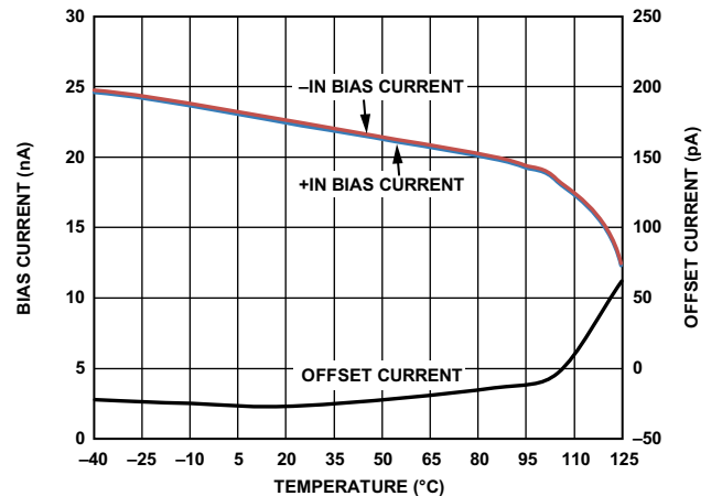
Figure 32. Input Bias Current and Input Offset Current vs. Temperature
