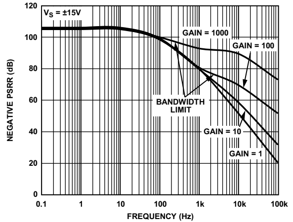
Figure 25. Negative PSRR vs. Frequency, RTI, V_S = \pm 15 V
