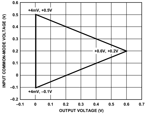
Figure 16. Input Common-Mode Voltage vs. Output Voltage, G = 1 , V_S = 2.7\text{ V}
