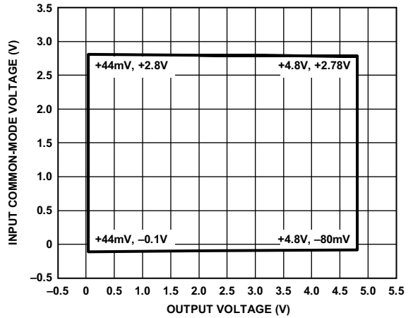
Figure 18. Input Common-Mode Voltage vs. Output Voltage, G = 100 , V_S = 5\text{ V}
