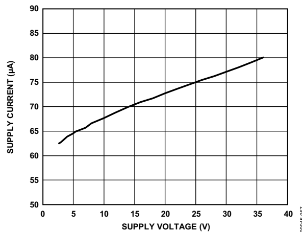
Figure 56. Supply Current vs. Supply Voltage
