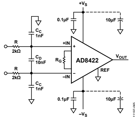
Figure 64. RFI Suppression
