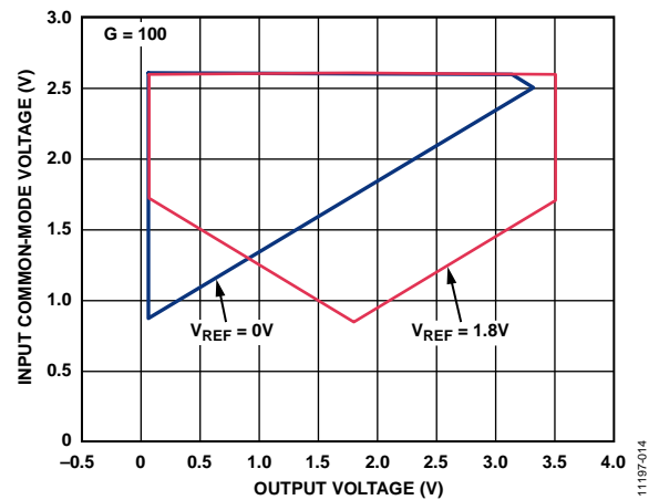
Figure 15. Input Common-Mode Voltage vs. Output Voltage ( G = 100 ), Single-Supply, V_S = 3.6V
