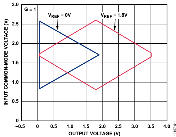
Figure 12. Input Common-Mode Voltage vs. Output Voltage ( G = 1 ), Single-Supply, V_S = 3.6V
