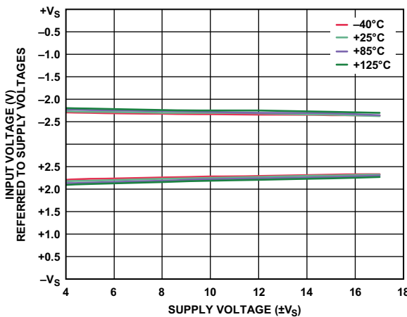
Figure 23. Input Voltage Limit vs. Supply Voltage
