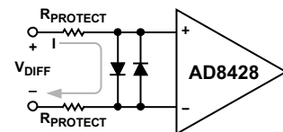
Figure 43. Protection for Large Differential Voltages
