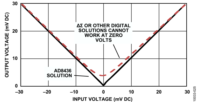
Figure 25. DC Transfer Function near Zero
