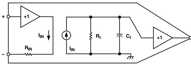
Figure 1. Equivalent Schematic
