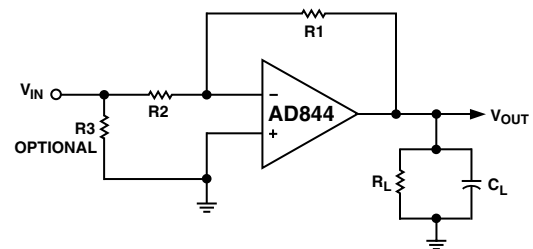
Figure 2. Inverting Amplifier
