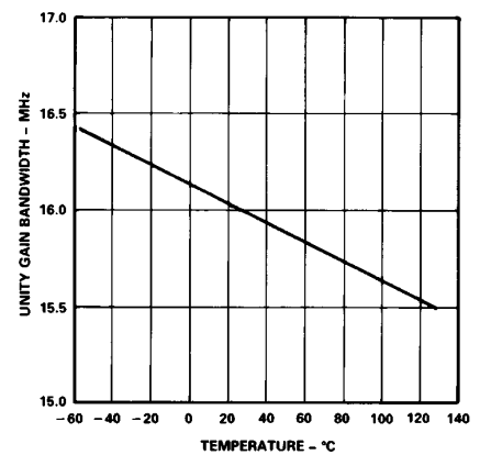
Figure 9. Unity-Gain Bandwidth
