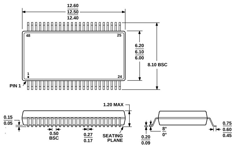
Figure 10. 48-Lead Thin Shrink Small Outline Package [TSSOP] (RU) Dimensions shown in millimeters
