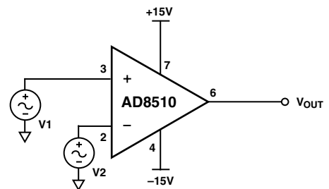
Figure 14. Pulsewidth Modulator
