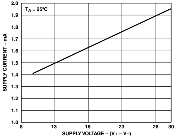
TPC 7. AD8512 Supply Current/Amplifier vs. Supply Voltage
