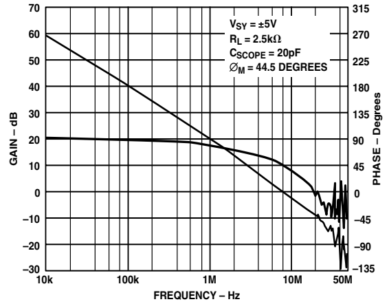
TPC 23. Open-Loop Gain and Phase vs. Frequency
