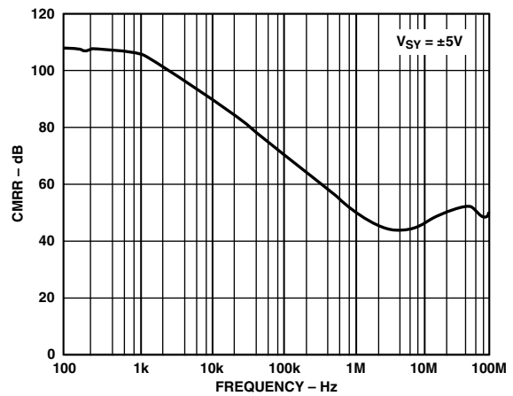
TPC 24. CMRR vs Frequency
