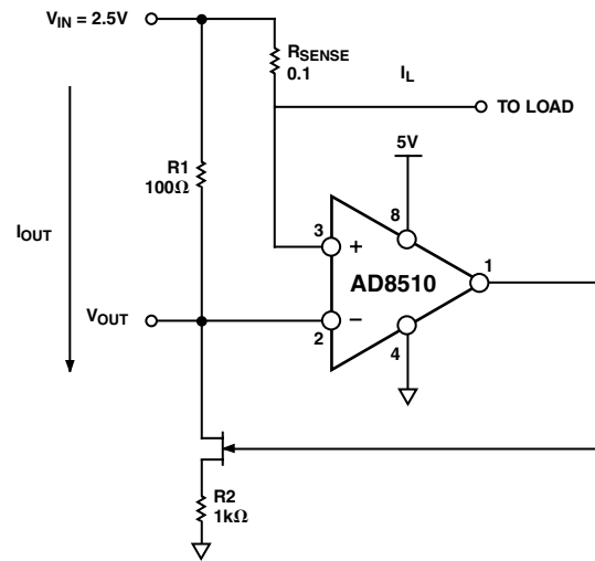
Figure 17. High Side Current Monitor
