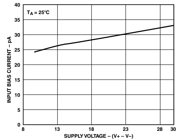
TPC 6. Input Bias Current vs. Supply Voltage
