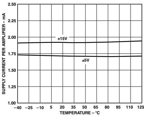
TPC 9. AD8512 Supply Current/Amplifier vs. Temperature
