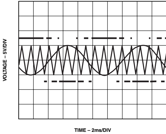
Figure 15. Pulsewidth Modulation
