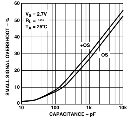
Figure 9. Small Signal Overshoot vs. Load Capacitance
