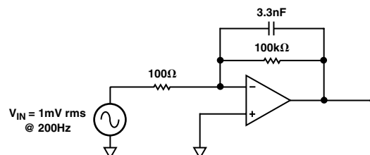
Figure 53a. Reducing Autocorrection Clock Noise with a Feedback Capacitor
