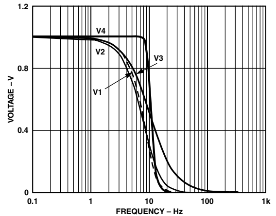
Figure 8. Frequency Response Output at Different Stages of the Low-Pass Filter
