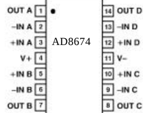
14-Lead SO (R-14)
