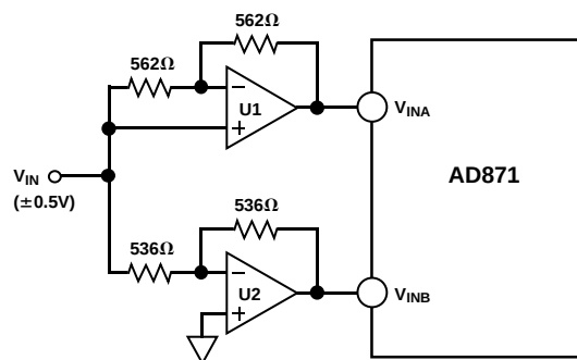
Figure 15. Single-Ended to Differential Connections; U1, U2 = AD811 or AD9617
