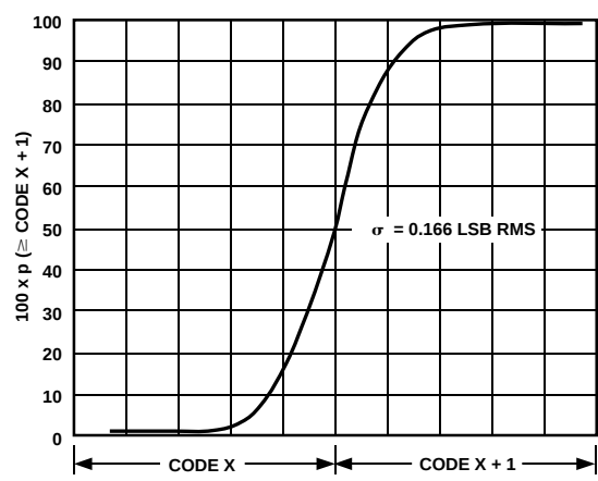
Figure 9. AD871 Code Probability at a Transition
