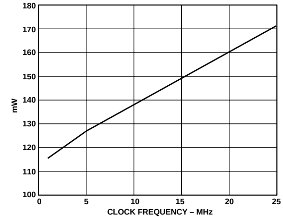
Figure 8. Power Consumption vs. Sample Rate
