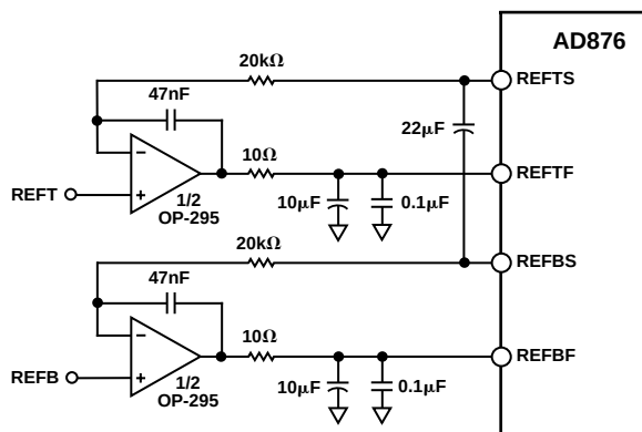
Figure 20. Kelvin Connected Reference Using the OP295
