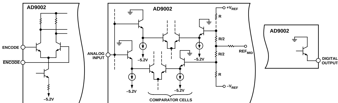
Figure 2. Input/Output Circuits
