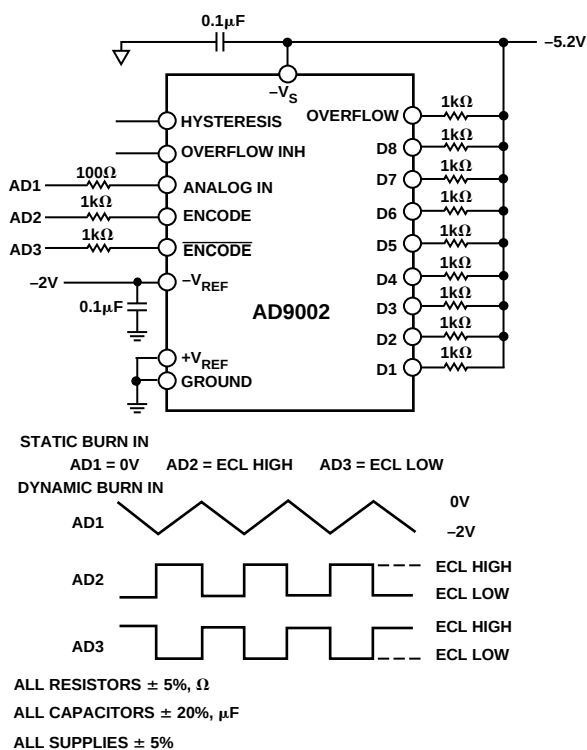
Figure 3. Burn-in Diagram
