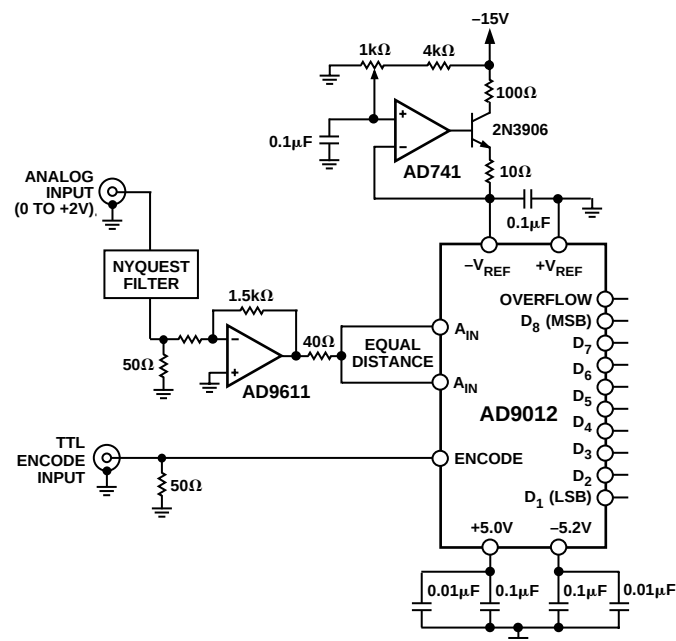
Figure 5. Typical Application
