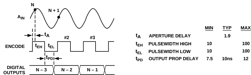
Figure 1. Timing Diagram
