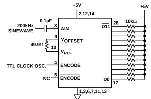
Figure 7. AD9042AD Burn-In Diagram
