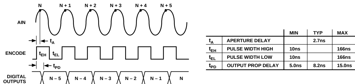
Figure 2. Timing Diagram
