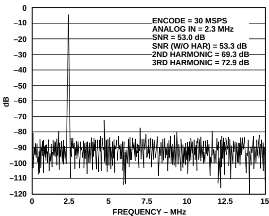
Figure 10. FFT Plot 30 MSPS, 2.3 MHz
