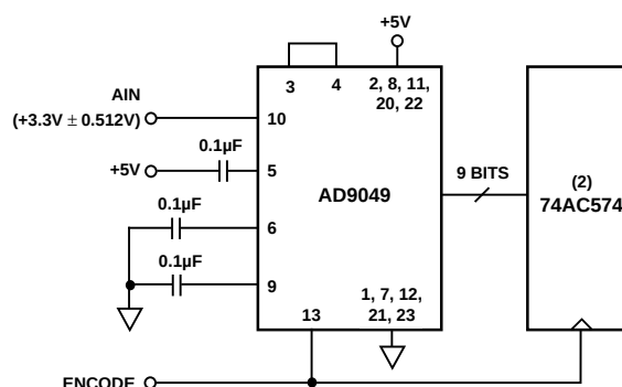
Figure 1. Typical Connections
