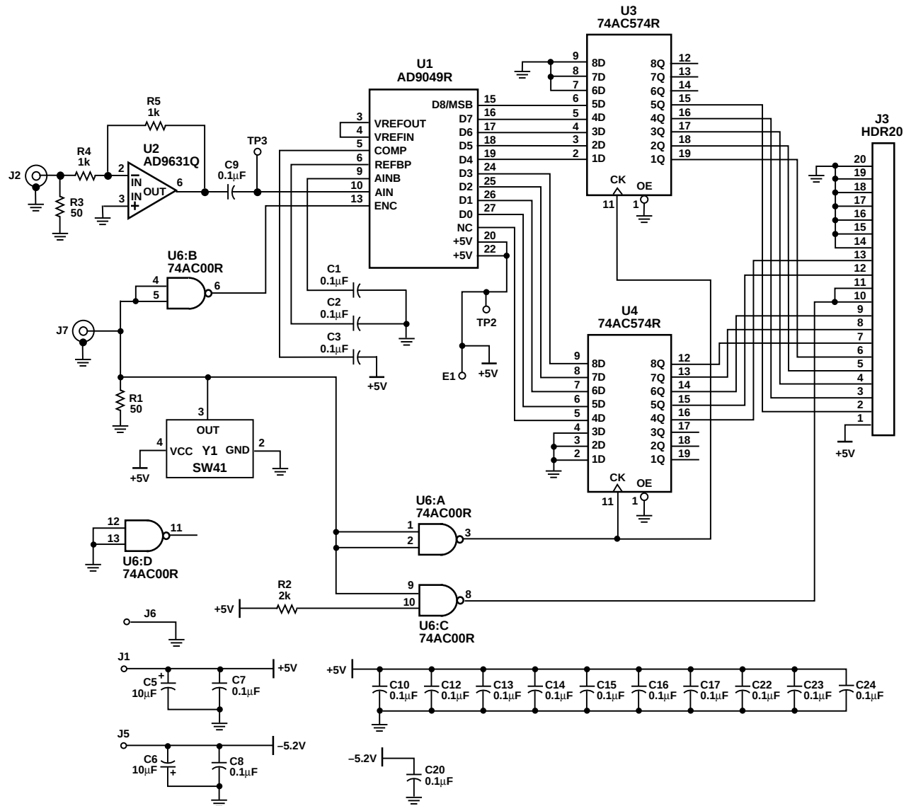
Figure 23. Evaluation Board Schematic
