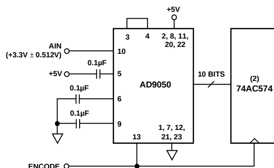
Figure 1. Typical Connections
