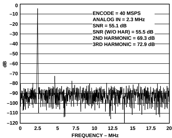
Figure 10. FFT Plot 40 MSPS, 2.3 MHz
