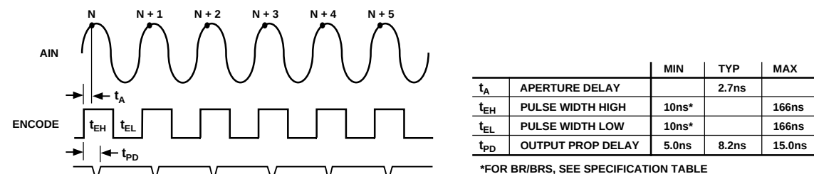
Figure 2. Timing Diagram
