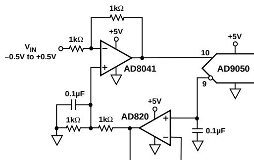
Figure 16. Single Supply, Single Ended, DC Coupled AD9050
