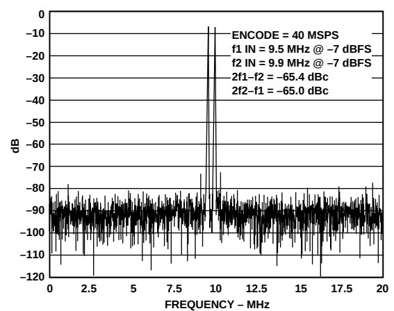
Figure 8. Two-Tone IMD
