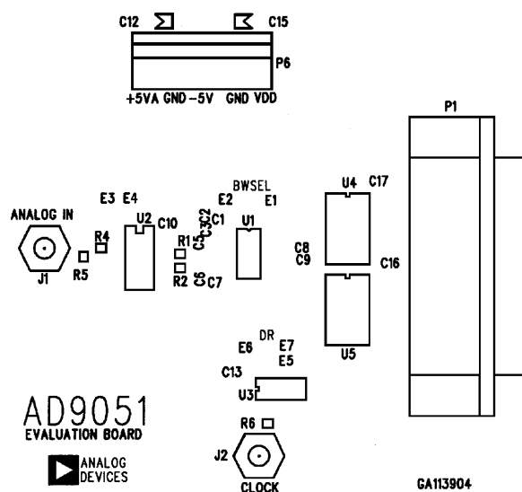
Figure 10. Silkscreen
