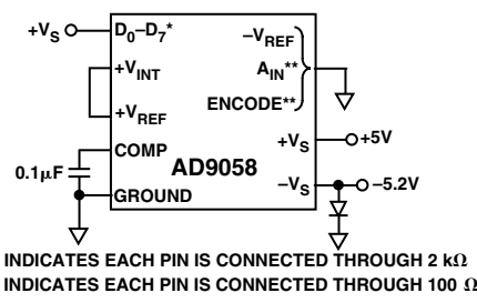
AD9058 Burn-In Connections
