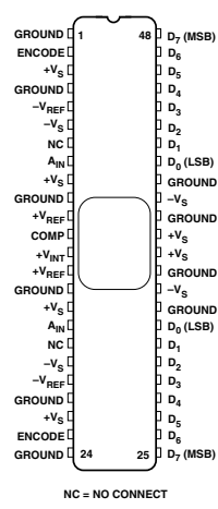
AD9058JD/KD Pinouts
