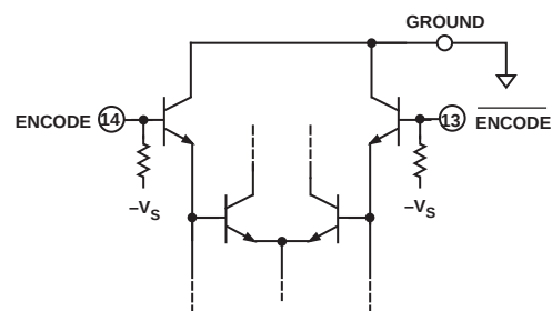
AD9060 Encode and \overline{\text{Encode}} Equivalant Circuits
