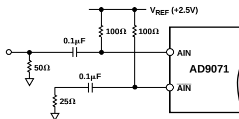
Figure 19. Single-Ended Analog Input Configuration
