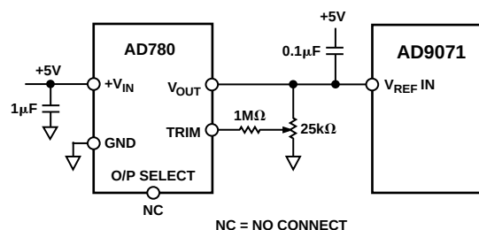
Figure 20. Using the AD780 Voltage Reference
