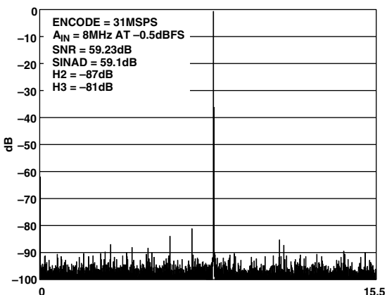
TPC 7. FFT: FS = 31 MSPS, A_{IN} = 8 MHz @ -0.5 dBFS, Differential, 1 V p-p Input Range
