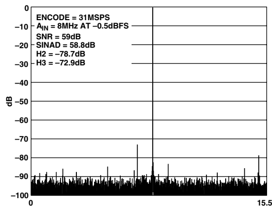
TPC 10. FFT: FS = 31 MSPS, A_{IN} = 8 MHz @ -0.5 dBFS; with AD8138 Driving ADC Inputs, 1 V p-p Input Range
