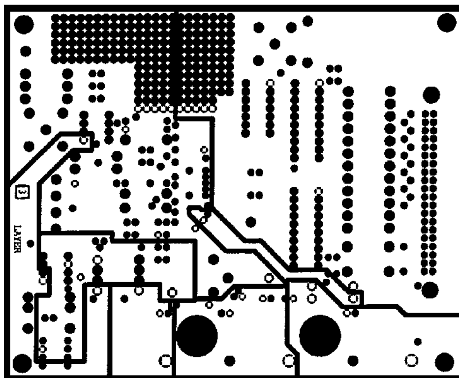
Figure 66. Evaluation Board Power Plane Layout
