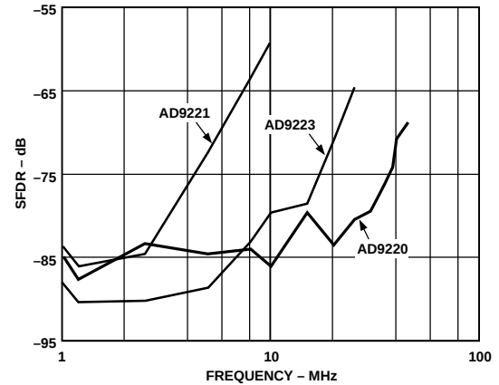
Figure 44. AD9221/AD9223/AD9220 SFDR vs. Input Frequency ( V_{CM} = 2.5\text{ V} , 2\text{ V p-p Input Span} , A_{IN} = -0.5\text{ dB} )
