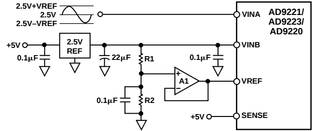
Figure 50. External Reference— V_{CM} = 2.5 V (2.5 V on VINB, Resistor Divider to Make VREF)
