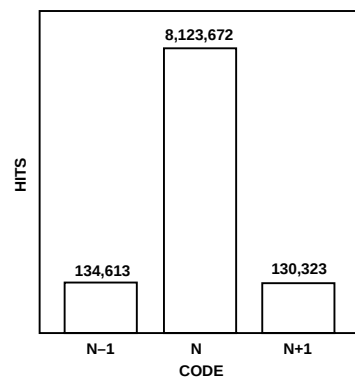
Figure 22. "Grounded-Input" Histogram (Input Span = 2 V p-p)
