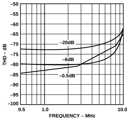
Figure 24. THD vs. Input Frequency (Input Span = 2.0 V p-p, V_{CM} = 2.5\text{ V} )
