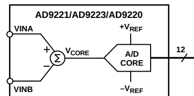
Figure 31. AD9221/AD9223/AD9220 Equivalent Functional Input Circuit
