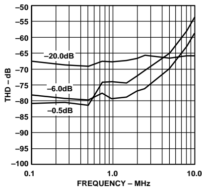
Figure 17. THD vs. Input Frequency (Input Span = 5.0 V p-p, V_{CM} = 2.5\text{ V} )
