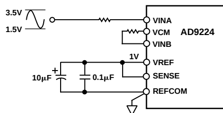
Figure 27. Internal Reference—2 V p-p Input Span, V_{CM} = 2.5 V
