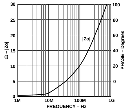
Figure 6. Output Impedance
