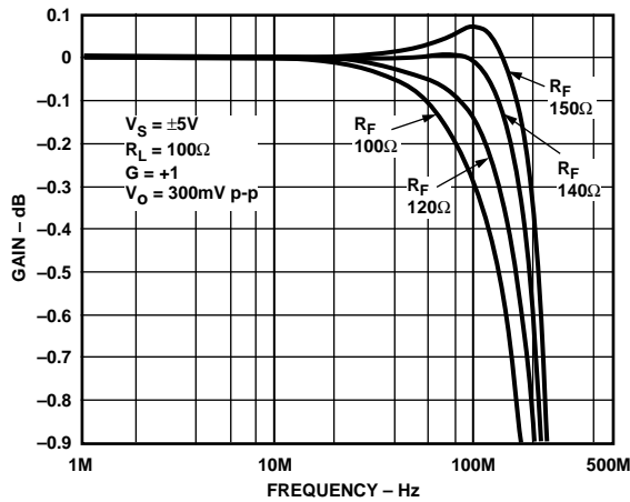
Figure 16. AD9631 0.1 dB Flatness, N Package (for R Package Add 20 Ω to R_F )
