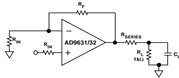
Figure 60. Driving Capacitive Loads
