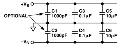
Supply Bypassing
