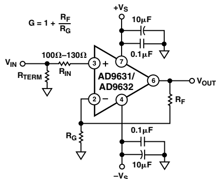
Figure 3. Noninverting Operation
