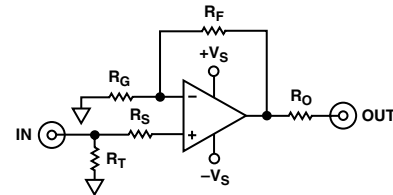
Noninverting Configuration
